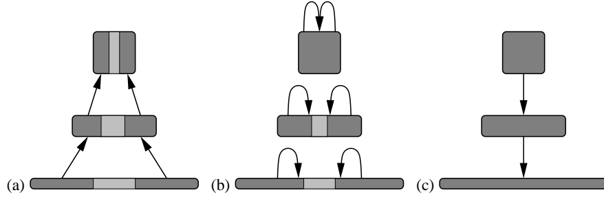
Fig. 1.13. Iterative image interpretation: (a) the image is interpreted first at positions where little ambiguity exists; (b) lateral interactions reduce ambiguity; (c) top-down expansion of abstract representations bias the low-level decision.
