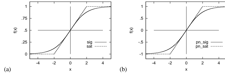
Fig. 4.5. Saturating transfer functions: (a) limiting the activities to the interval [0, 1] ( f_{sat} : \alpha = 2 ; f_{sig} : \beta = 1 ); (b) limiting the activities to [-1, 1] ( f_{pn\_sat} : \alpha = 2 ; f_{pn\_sig} : \beta = 1 ).
