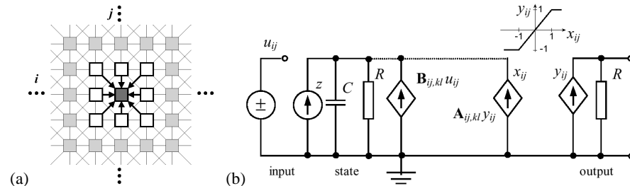
Fig. 3.14. Cellular neural network model of Chua and Roska [41, 42]: (a) processing elements are arranged in a grid and connected locally; (b) core cell of continuous time analog CNN.
