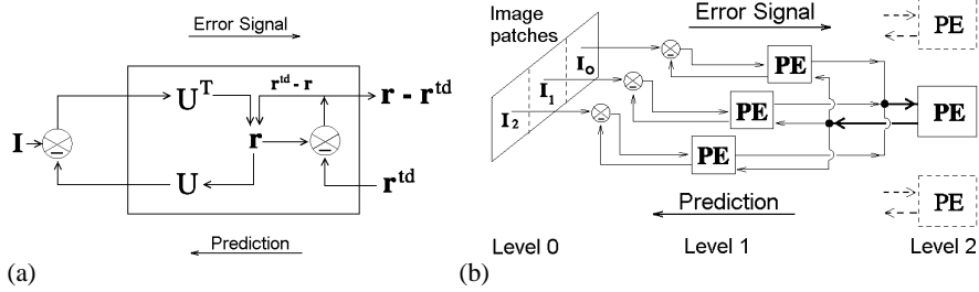
Fig. 3.11. Hierarchical Kalman filter proposed by Rao and Ballard [187]: (a) predictive estimator (PE) module that integrates top-down predictions \mathbf{r}^{td} and a feed-forward error signal ( I - U\mathbf{r} ) to an estimate \mathbf{r} of the causes of an image I ; matrix U mediates between the image and the causes; (b) general architecture of the system: local PEs are combined by a higher-level PE (images adapted from [187]).
