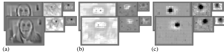
Fig. 10.6. Face localization recall. Shown are the contributions to the activity of the network's output units after iteration 10 of Fig. 10.5 (bright shading represents inhibition, dark shading indicates excitation): (a) via input and forward projections; (b) via lateral projections; (c) via backward projections.
