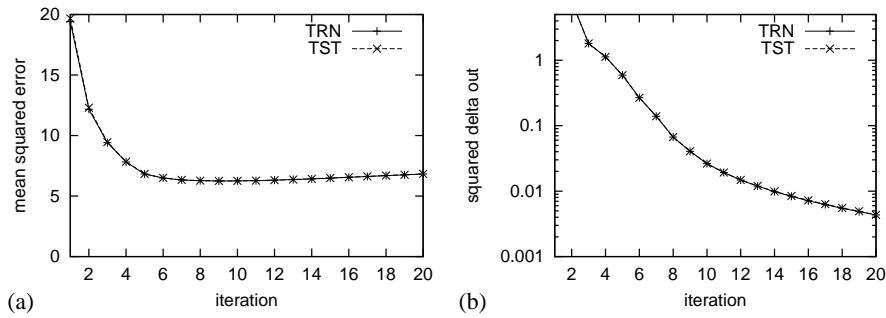
Fig. 9.16. Filling-in of occlusions – performance over time: (a) mean squared error; (b) mean square delta output.
