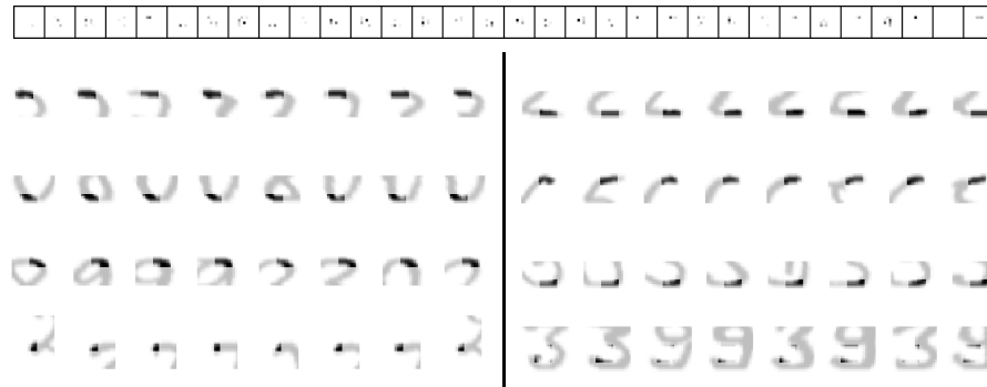
Fig. 5.4. Learning a hierarchy of sparse features – stroke features. Shown are the eight best stimuli of eight features that detect horizontal strokes with different curvature. The upper part of the figure shows the sparse activity of all 32 stroke features.
